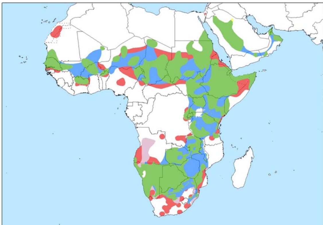
Figure 17: Distribution map of the Lappet-faced Vulture Torgos tracheliotos .
